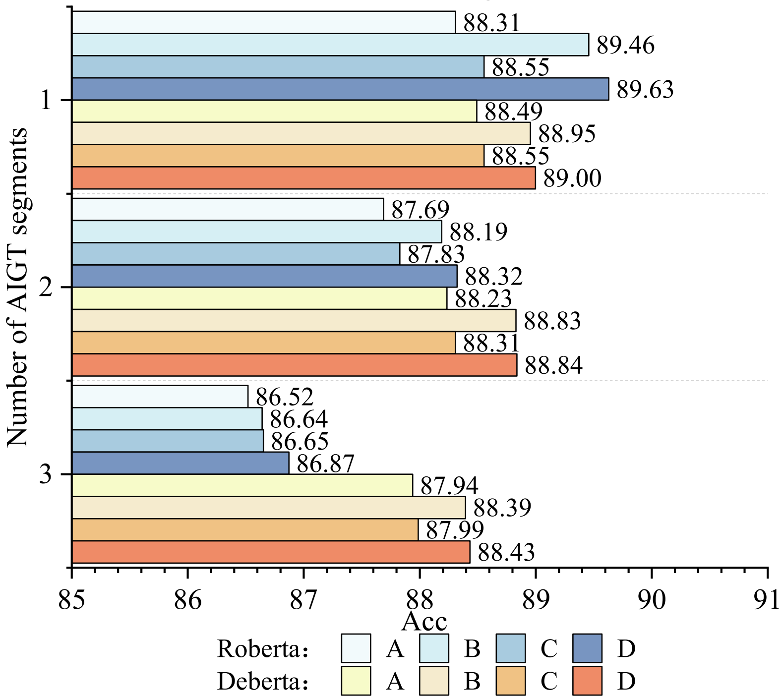
Acc based on GPT-J generated text
